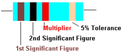
Typical 4 band Resistor
